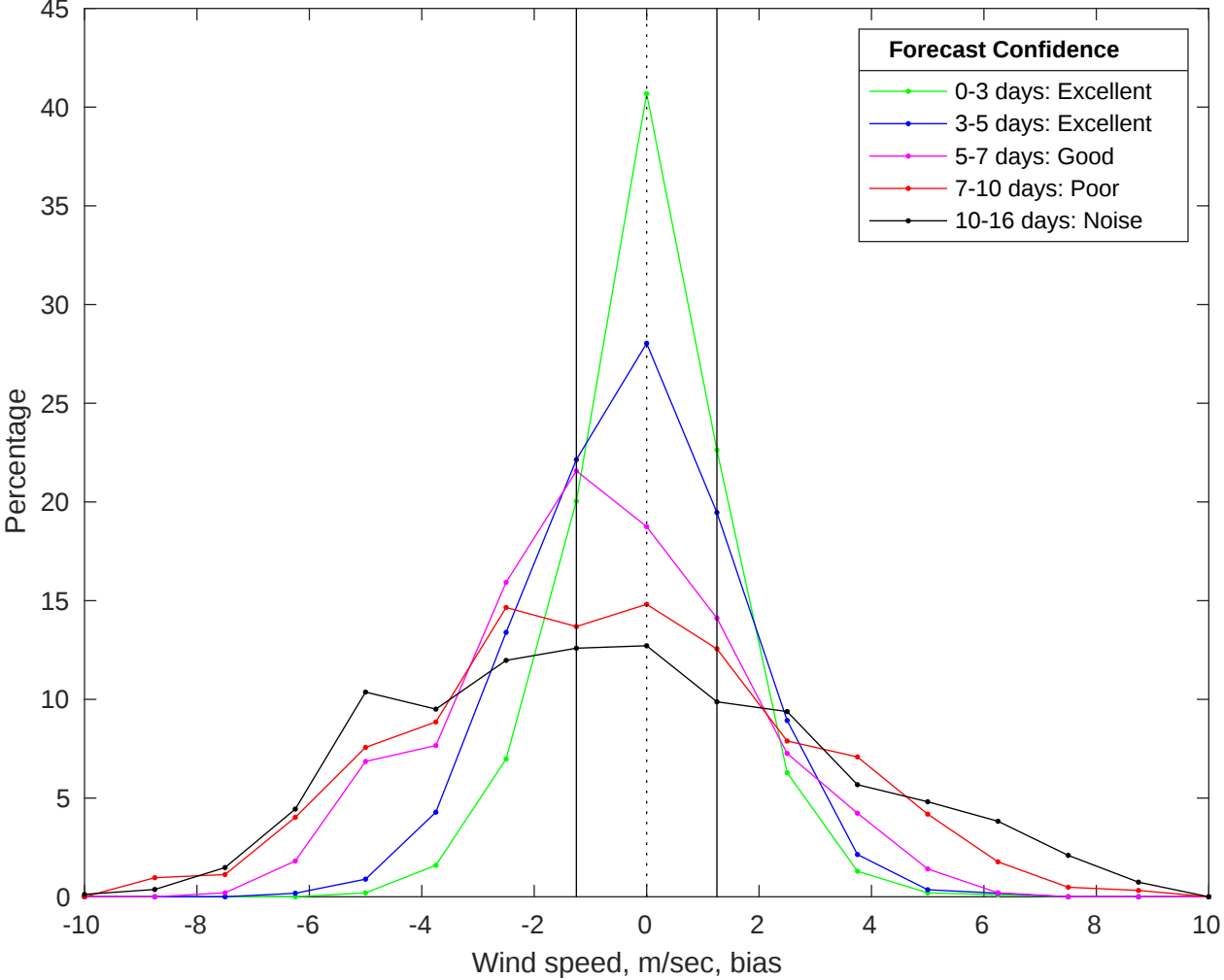
NDBC 46059 vs GFS Winds Bias Histogram: 29-Jan-2026
