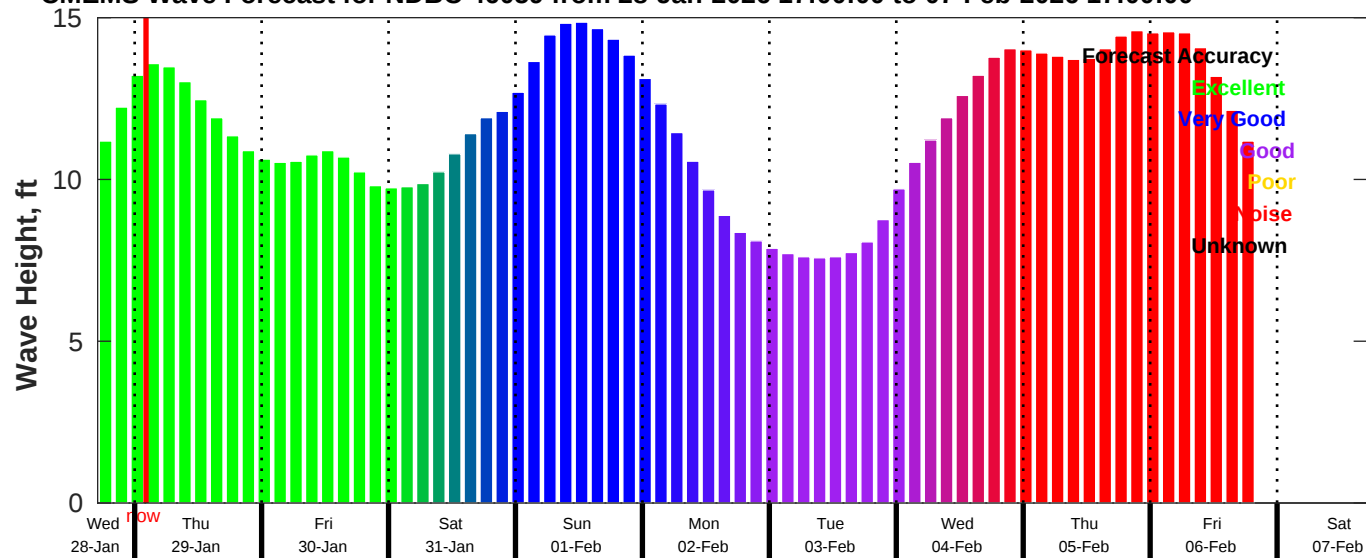
CMEMS Wave Forecast for NDBC 46059 from 28-Jan-2026 17:00:00 to 07-Feb-2026 17:00:00
