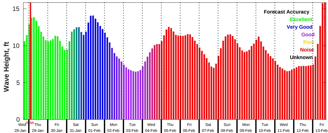
GFS Wave Forecast for NDBC 46059 from 28-Jan-2026 17:00:00 to 13-Feb-2026 17:00:00
