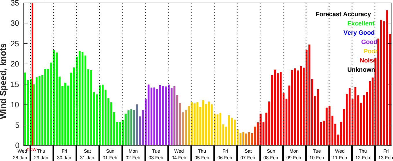
GFS Wind Speed Forecast for NDBC 46059 from 28-Jan-2026 17:00:00 to 13-Feb-2026 17:00:00
