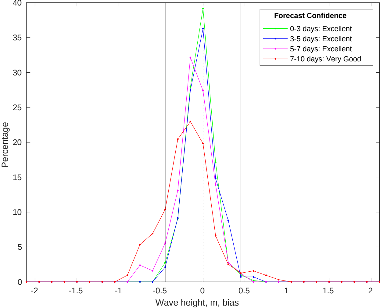
NDBC 46069 vs CMEMS Waves Bias Histogram: 29-Jan-2026
