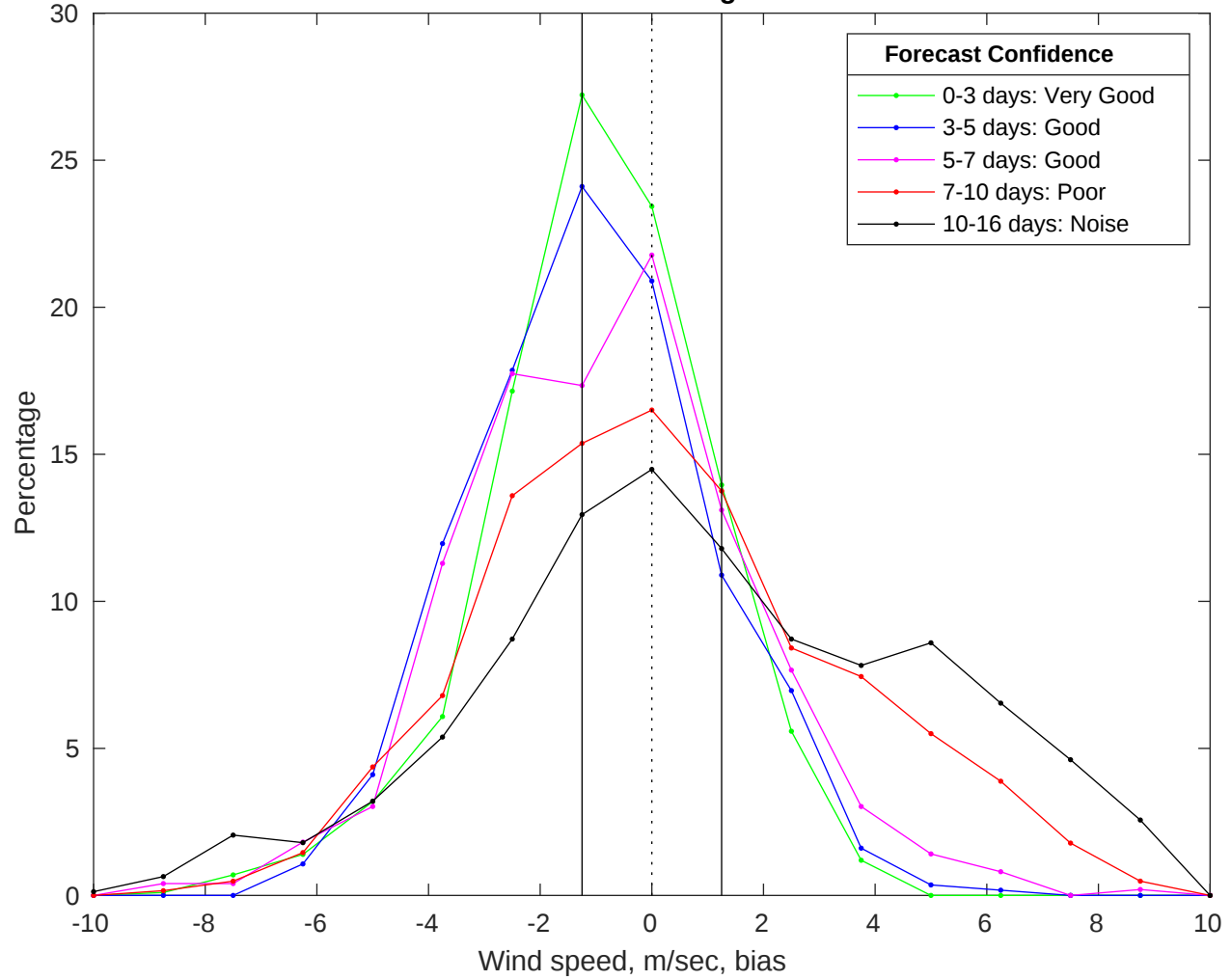
NDBC 46069 vs GFS Winds Bias Histogram: 29-Jan-2026
