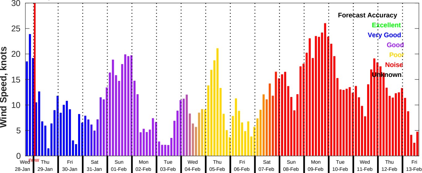
GFS Wind Speed Forecast for NDBC 46069 from 28-Jan-2026 16:00:00 to 13-Feb-2026 16:00:00
