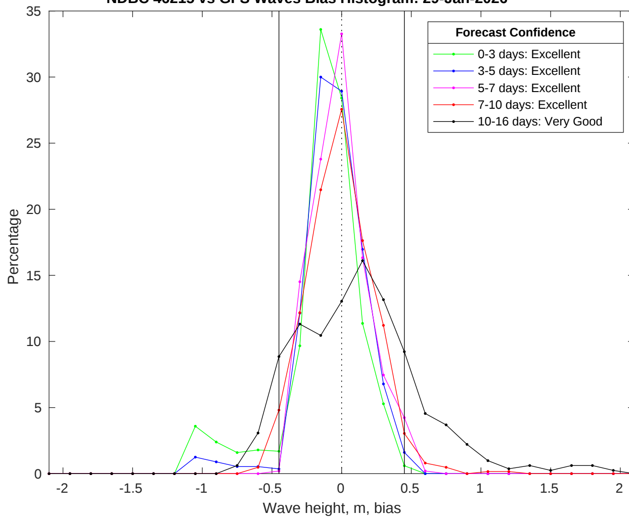
NDBC 46215 vs GFS Waves Bias Histogram: 29-Jan-2026
