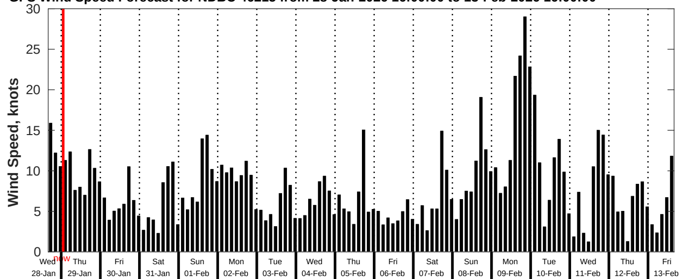
GFS Wind Speed Forecast for NDBC 46215 from 28-Jan-2026 16:00:00 to 13-Feb-2026 16:00:00
