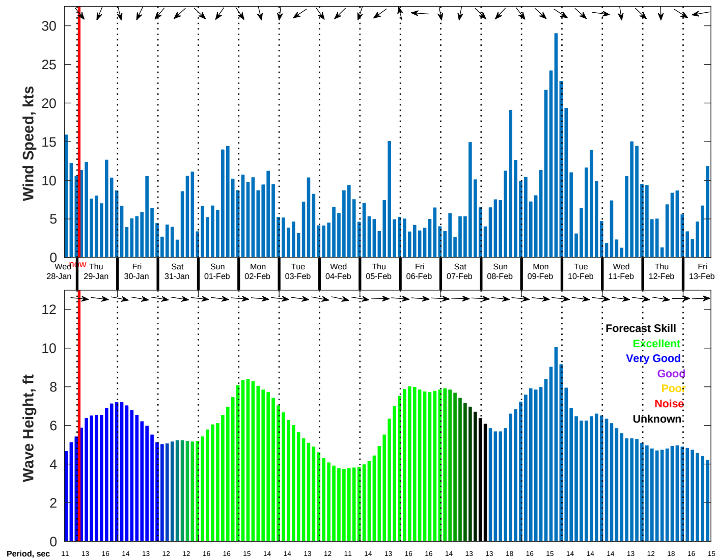
Wind & Wave Forecast for NDBC 46215 from 28-Jan-2026 16:00:00 to 13-Feb-2026 16:00:00
