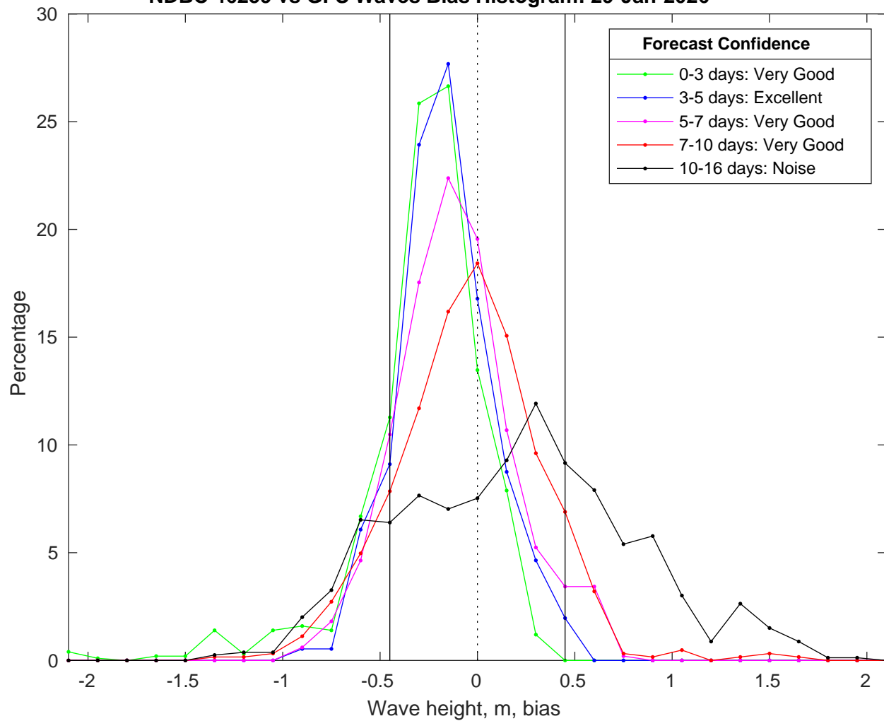
NDBC 46259 vs GFS Waves Bias Histogram: 29-Jan-2026
