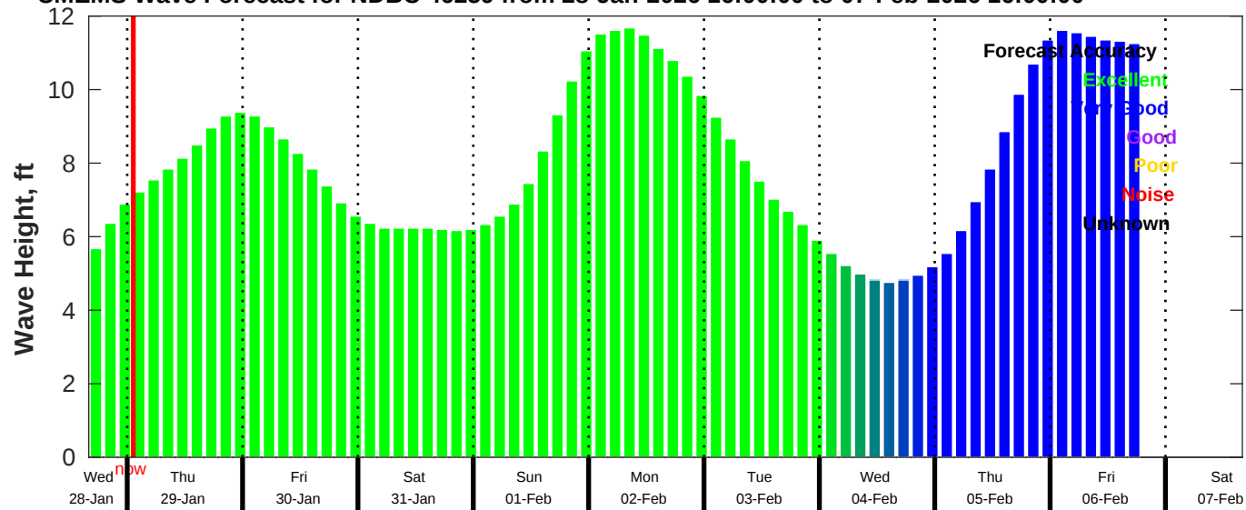
CMEMS Wave Forecast for NDBC 46259 from 28-Jan-2026 16:00:00 to 07-Feb-2026 16:00:00
