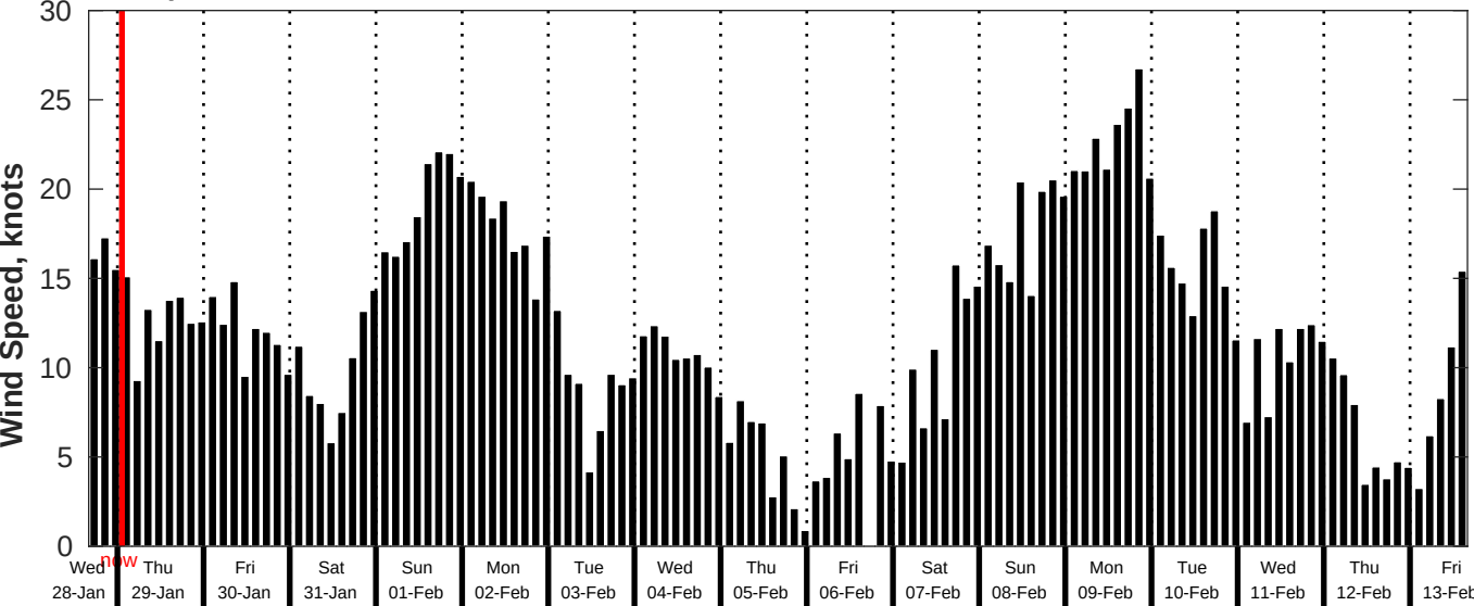
GFS Wind Speed Forecast for NDBC 46259 from 28-Jan-2026 16:00:00 to 13-Feb-2026 16:00:00
