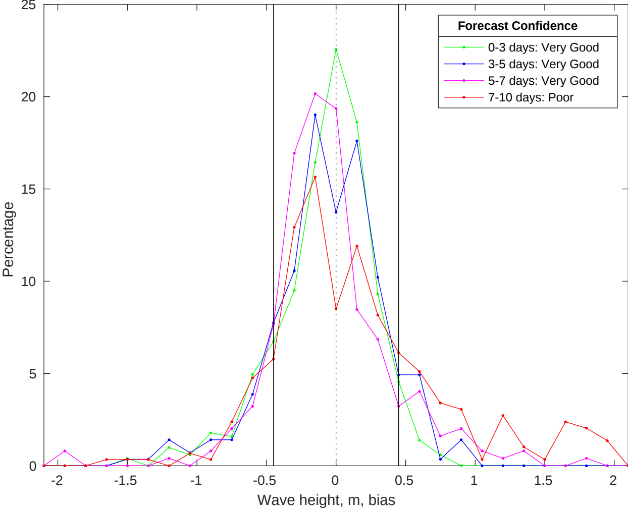
NDBC 51000 vs CMEMS Waves Bias Histogram: 29-Jan-2026
