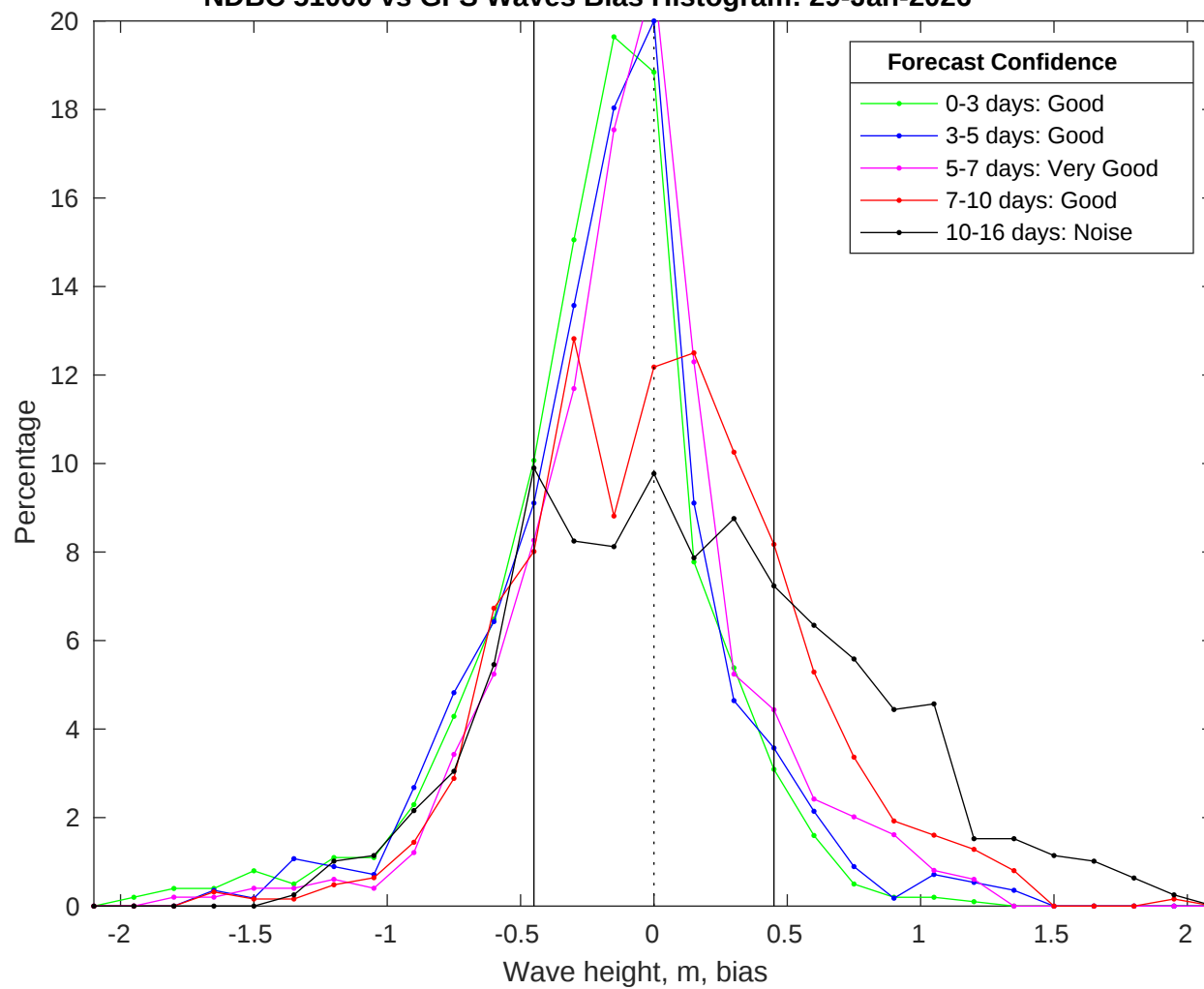
NDBC 51000 vs GFS Waves Bias Histogram: 29-Jan-2026
