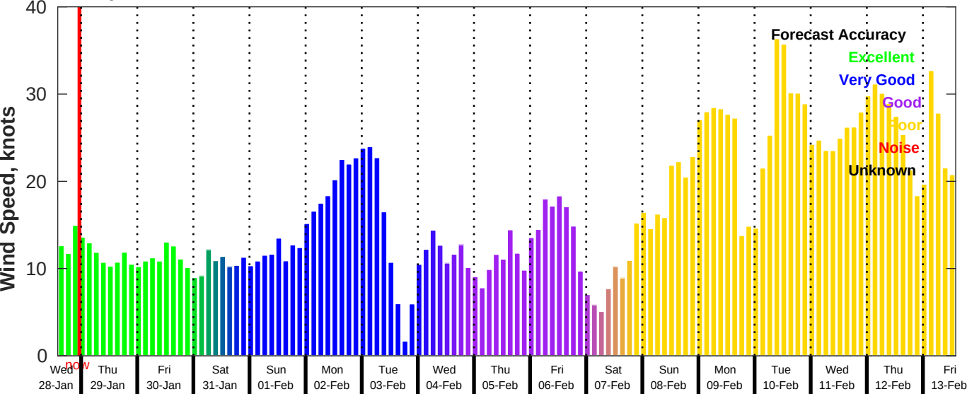
GFS Wind Speed Forecast for NDBC 51000 from 28-Jan-2026 14:00:00 to 13-Feb-2026 14:00:00
