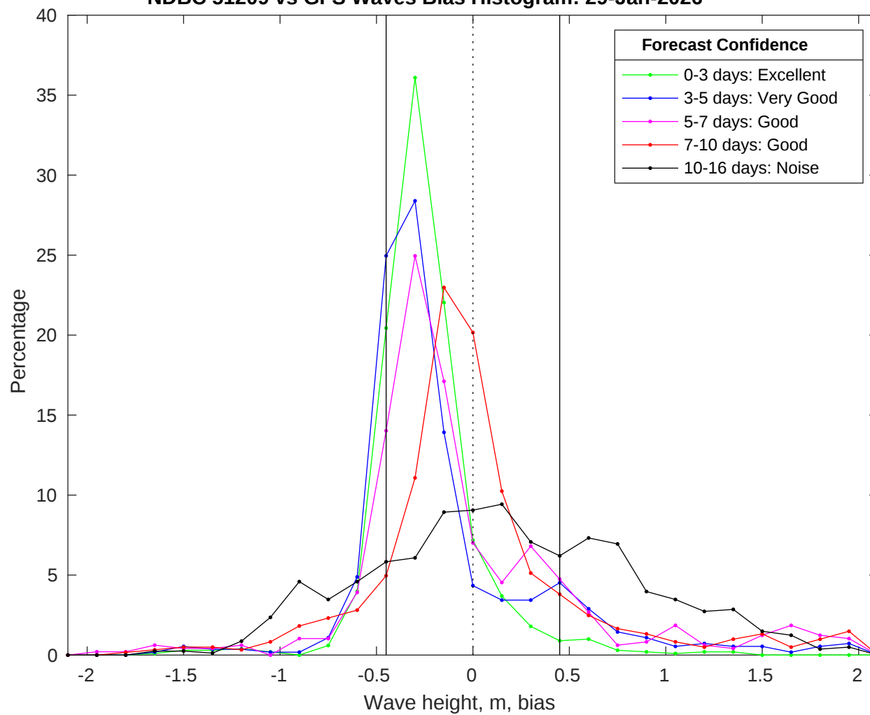
NDBC 51209 vs GFS Waves Bias Histogram: 29-Jan-2026
