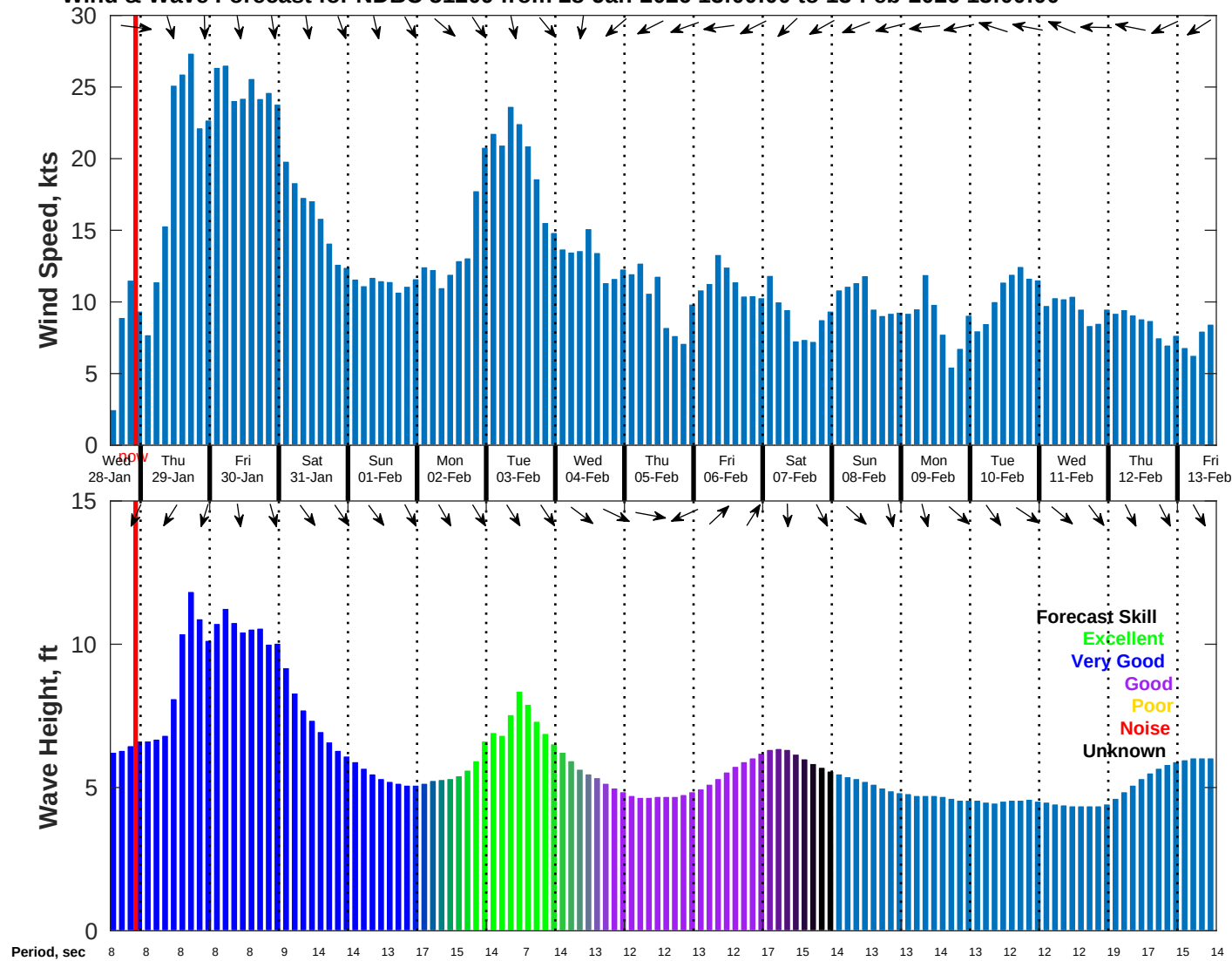
Wind & Wave Forecast for NDBC 51209 from 28-Jan-2026 13:00:00 to 13-Feb-2026 13:00:00
