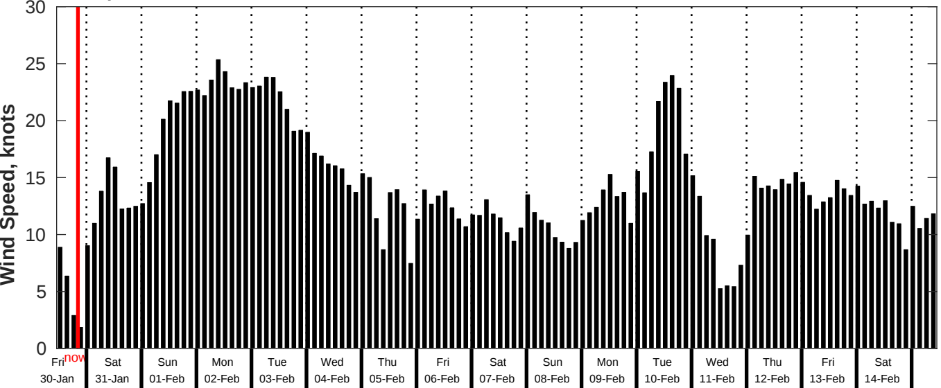
GFS Wind Speed Forecast for NDBC 52211 from 29-Jan-2026 11:00:00 to 14-Feb-2026 11:00:00
