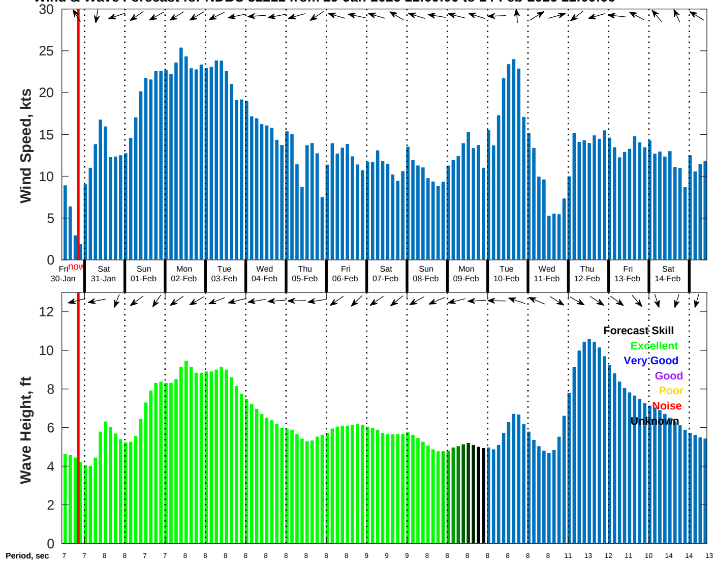
Wind & Wave Forecast for NDBC 52211 from 29-Jan-2026 11:00:00 to 14-Feb-2026 11:00:00
