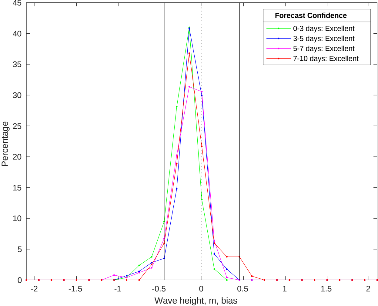
NDBC 52213 vs CMEMS Waves Bias Histogram: 29-Jan-2026
