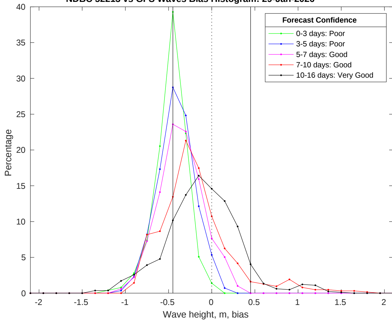
NDBC 52213 vs GFS Waves Bias Histogram: 29-Jan-2026
