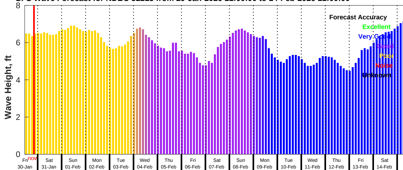
GFS Wave Forecast for NDBC 52213 from 29-Jan-2026 11:00:00 to 14-Feb-2026 11:00:00
