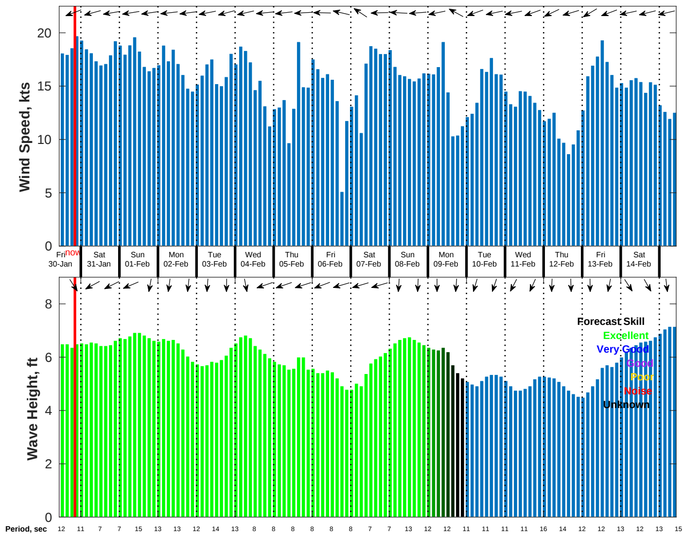
Wind & Wave Forecast for NDBC 52213 from 29-Jan-2026 11:00:00 to 14-Feb-2026 11:00:00
