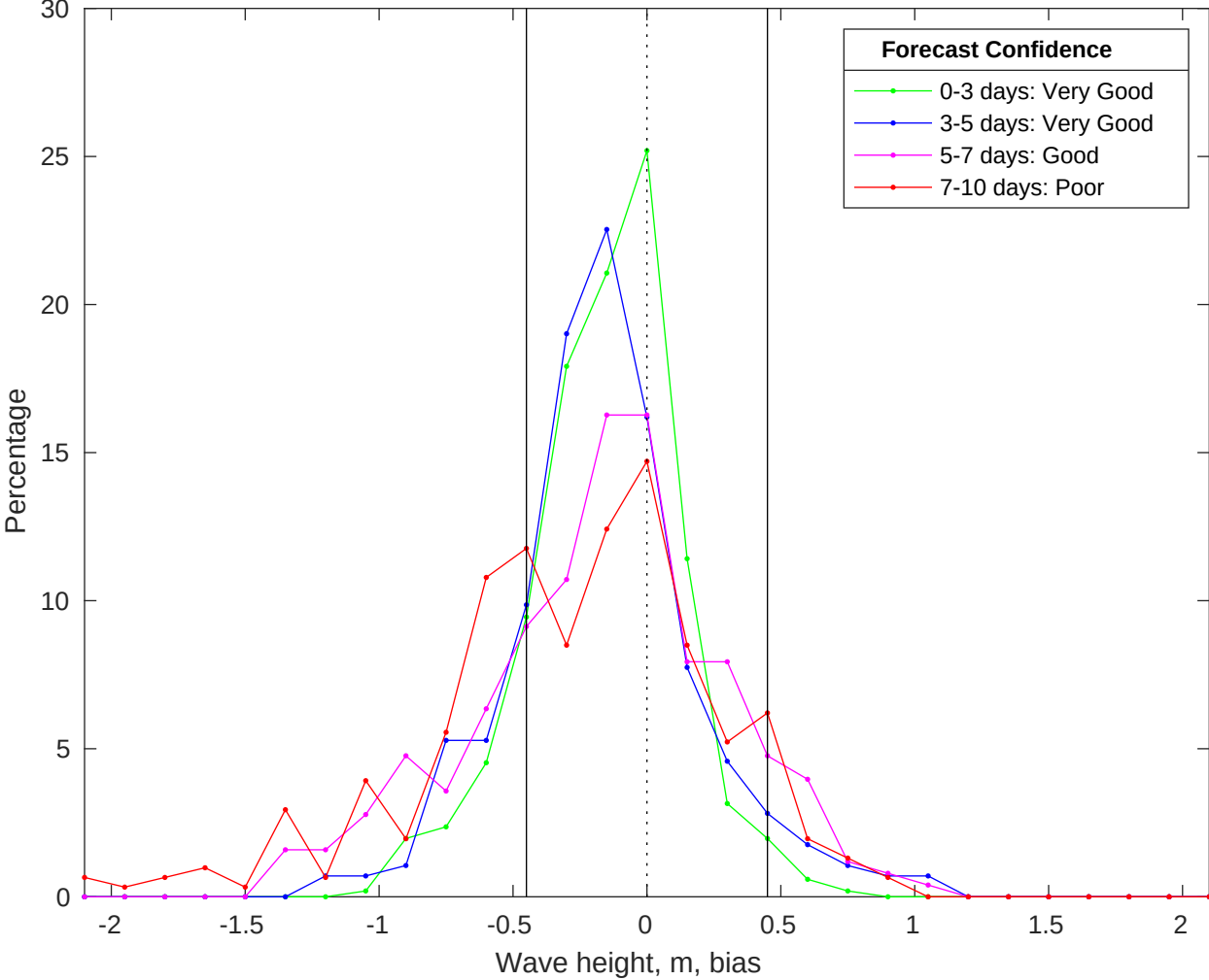
NDBC 41004 vs CMEMS Waves Bias Histogram: 30-Jan-2026
