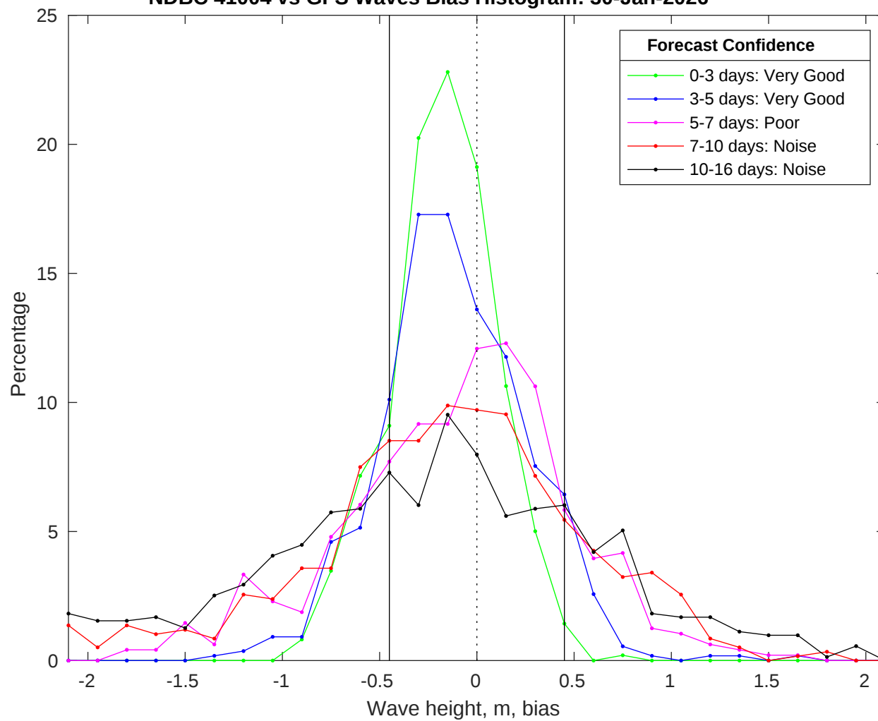
NDBC 41004 vs GFS Waves Bias Histogram: 30-Jan-2026
