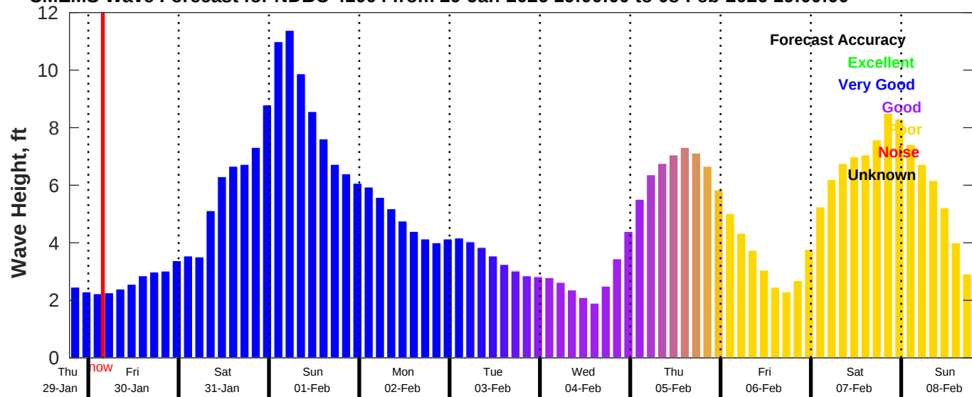
CMEMS Wave Forecast for NDBC 41004 from 29-Jan-2026 19:00:00 to 08-Feb-2026 19:00:00
