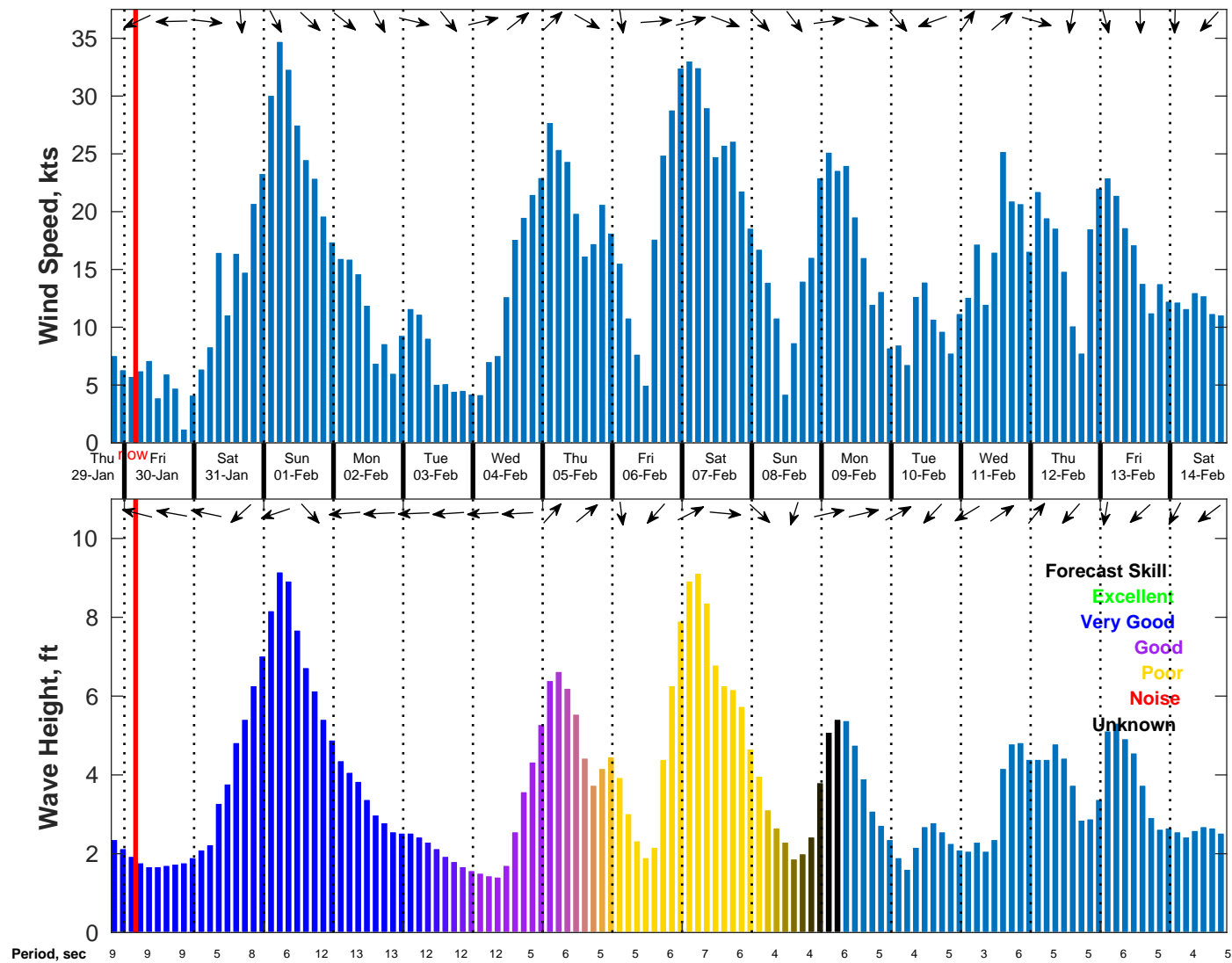
Wind & Wave Forecast for NDBC 41004 from 29-Jan-2026 19:00:00 to 14-Feb-2026 19:00:00
