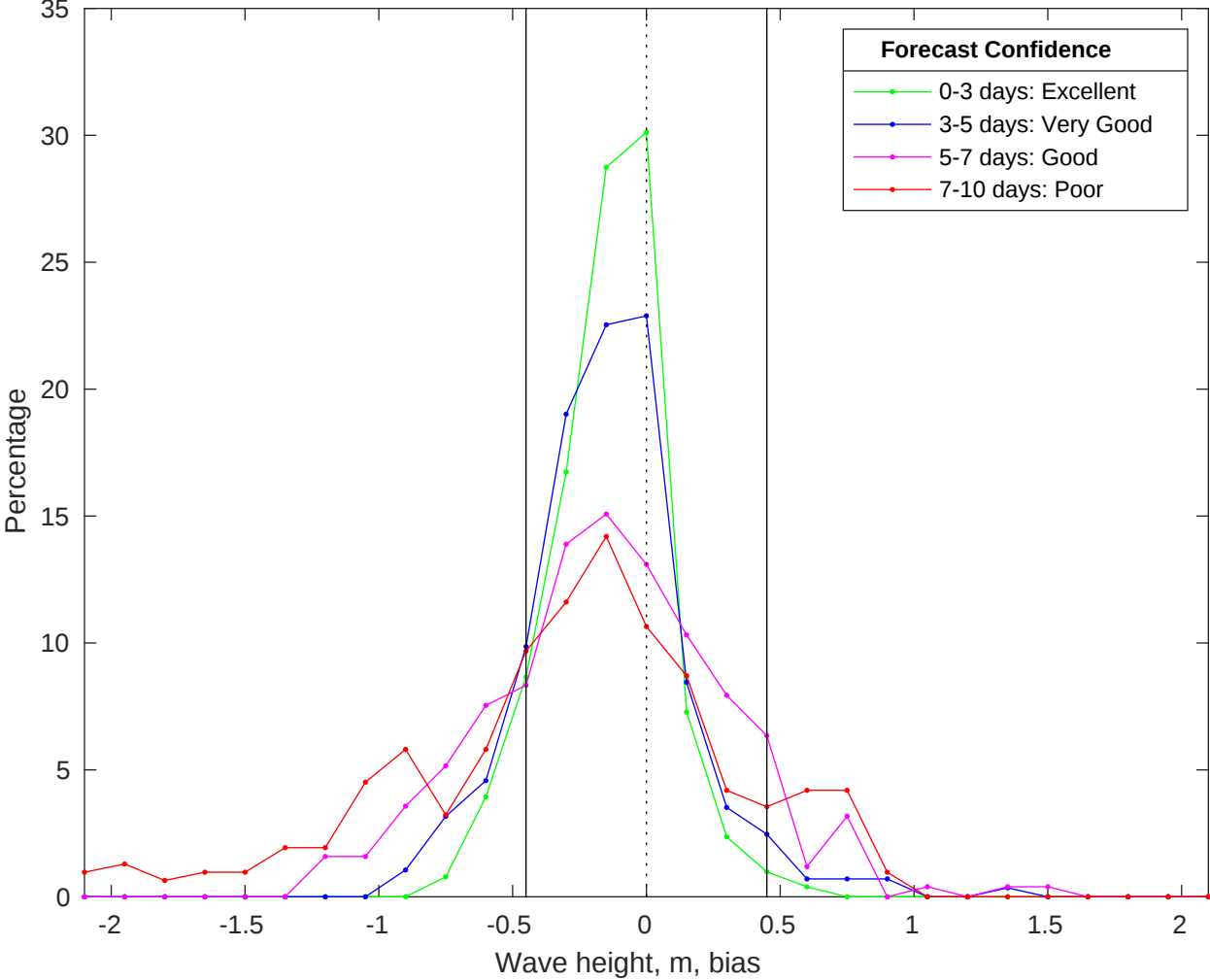
NDBC 41013 vs CMEMS Waves Bias Histogram: 30-Jan-2026
