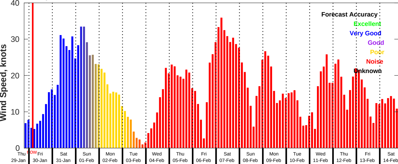
GFS Wind Speed Forecast for NDBC 41013 from 29-Jan-2026 19:00:00 to 14-Feb-2026 19:00:00
