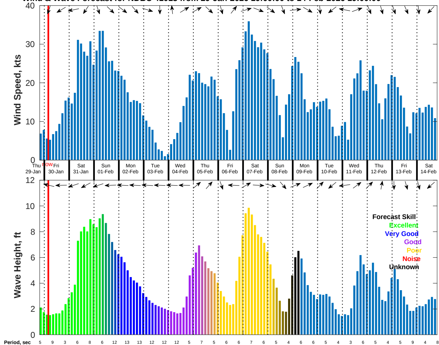
Wind & Wave Forecast for NDBC 41013 from 29-Jan-2026 19:00:00 to 14-Feb-2026 19:00:00
