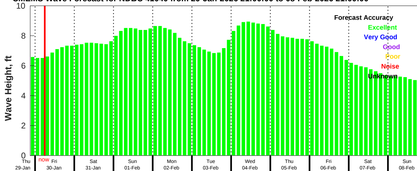
CMEMS Wave Forecast for NDBC 41040 from 29-Jan-2026 21:00:00 to 08-Feb-2026 21:00:00
