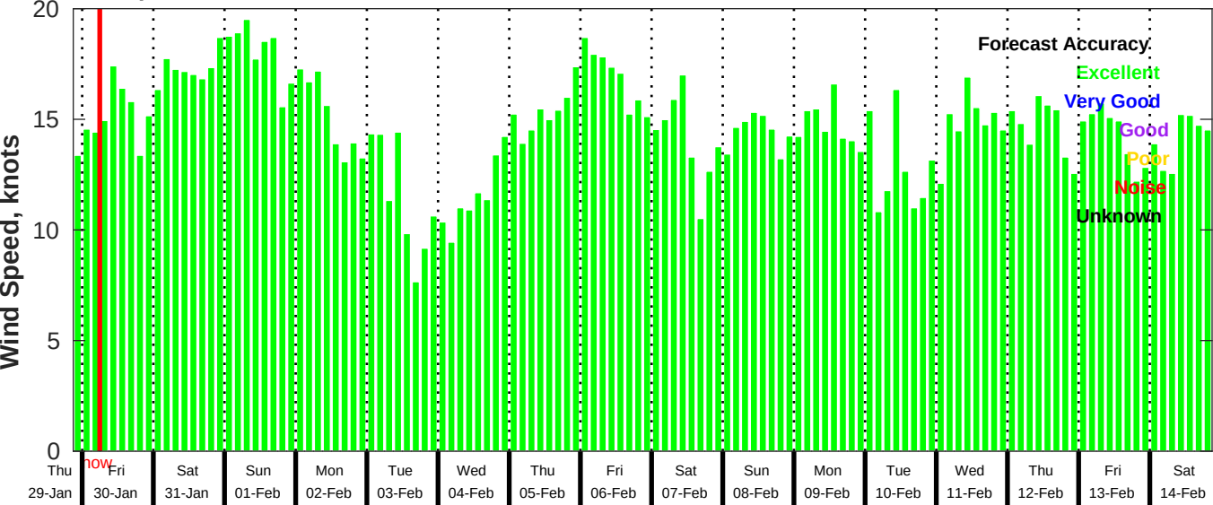
GFS Wind Speed Forecast for NDBC 41040 from 29-Jan-2026 21:00:00 to 14-Feb-2026 21:00:00
