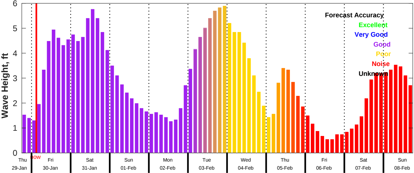
CMEMS Wave Forecast for NDBC 42019 from 29-Jan-2026 18:00:00 to 08-Feb-2026 18:00:00
