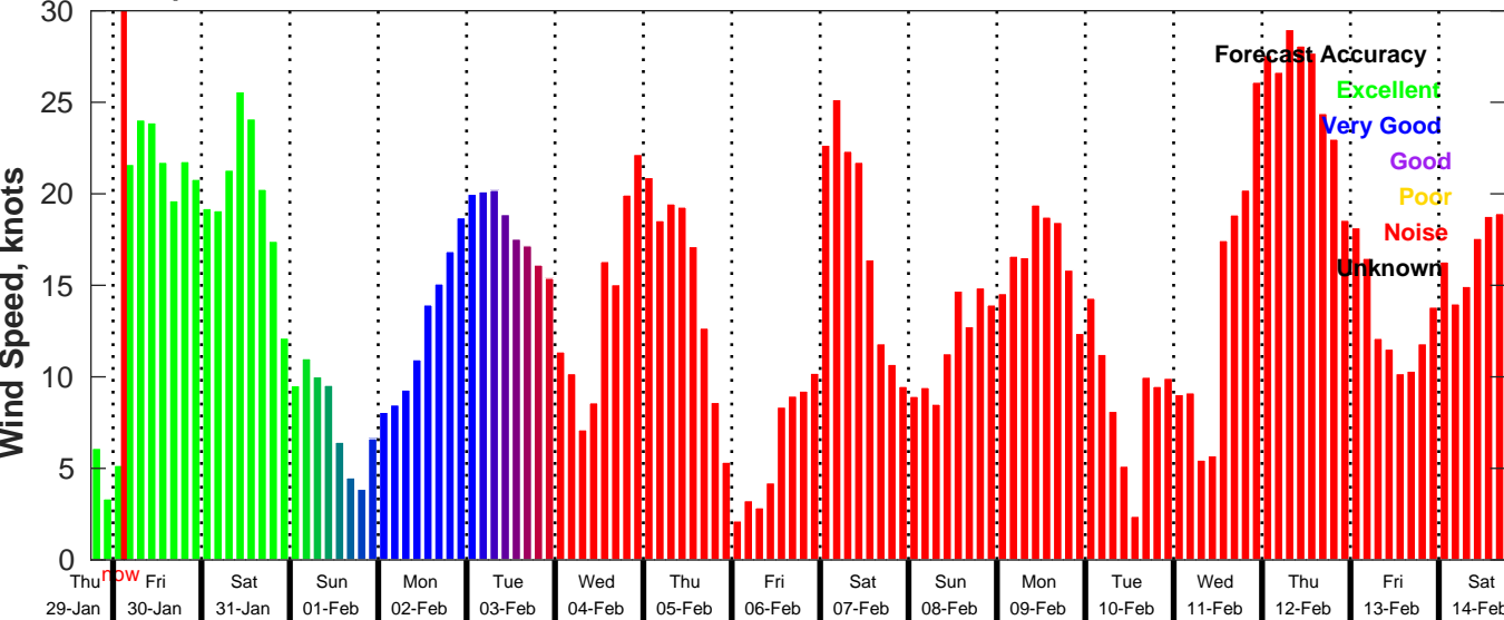
GFS Wind Speed Forecast for NDBC 42019 from 29-Jan-2026 18:00:00 to 14-Feb-2026 18:00:00
