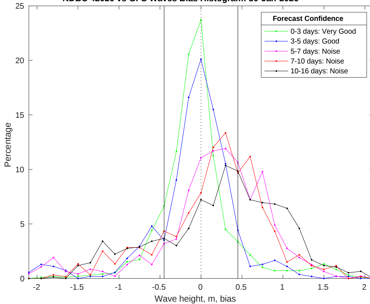
NDBC 42020 vs GFS Waves Bias Histogram: 30-Jan-2026
