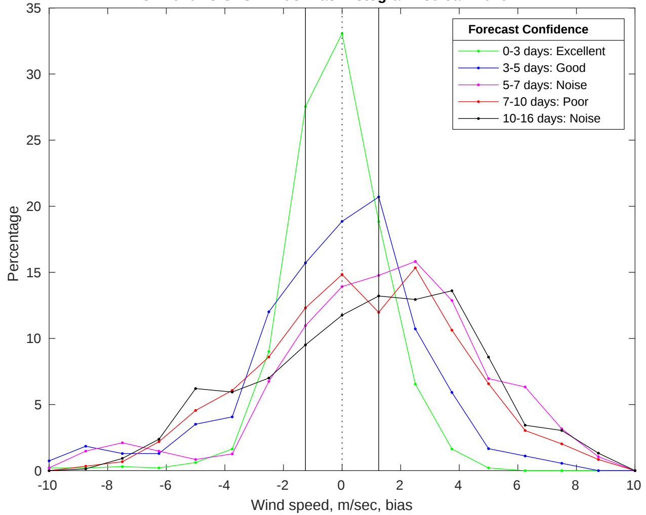
NDBC 42020 vs GFS Winds Bias Histogram: 30-Jan-2026
