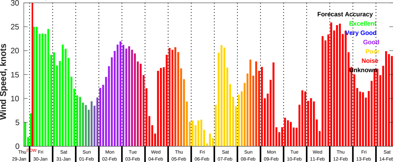
GFS Wind Speed Forecast for NDBC 42020 from 29-Jan-2026 18:00:00 to 14-Feb-2026 18:00:00
