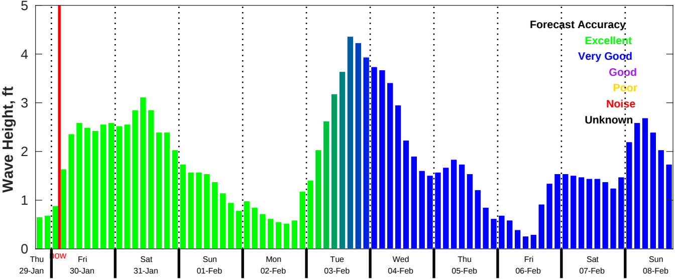
CMEMS Wave Forecast for NDBC 42035 from 29-Jan-2026 18:00:00 to 08-Feb-2026 18:00:00
