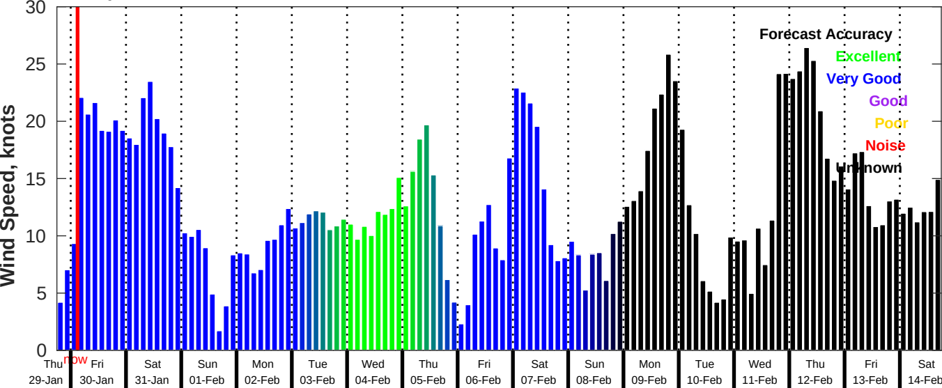
GFS Wind Speed Forecast for NDBC 42035 from 29-Jan-2026 18:00:00 to 14-Feb-2026 18:00:00
