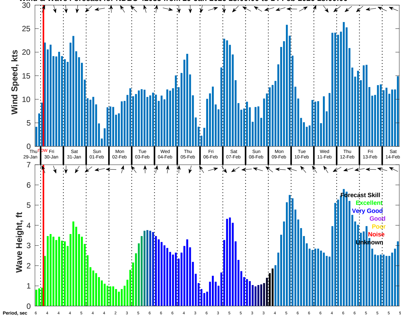
Wind & Wave Forecast for NDBC 42035 from 29-Jan-2026 18:00:00 to 14-Feb-2026 18:00:00
