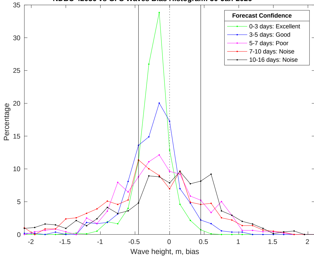
NDBC 42036 vs GFS Waves Bias Histogram: 30-Jan-2026
