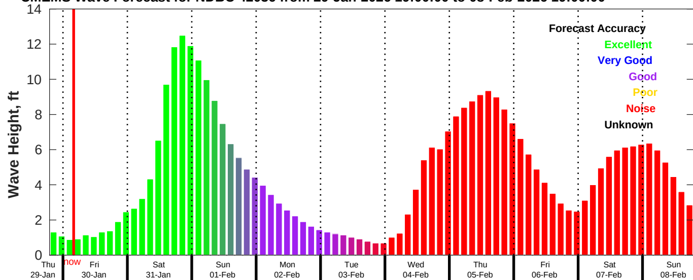
CMEMS Wave Forecast for NDBC 42036 from 29-Jan-2026 19:00:00 to 08-Feb-2026 19:00:00
