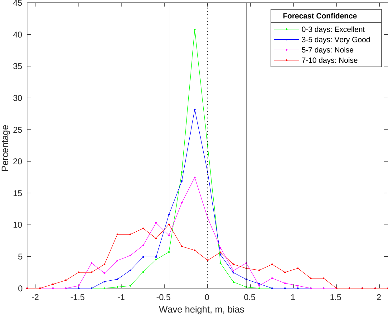
NDBC 42040 vs CMEMS Waves Bias Histogram: 30-Jan-2026
