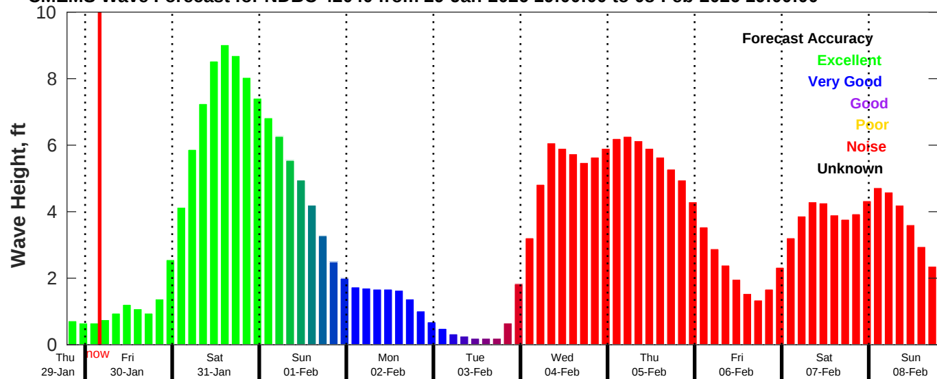
CMEMS Wave Forecast for NDBC 42040 from 29-Jan-2026 19:00:00 to 08-Feb-2026 19:00:00
