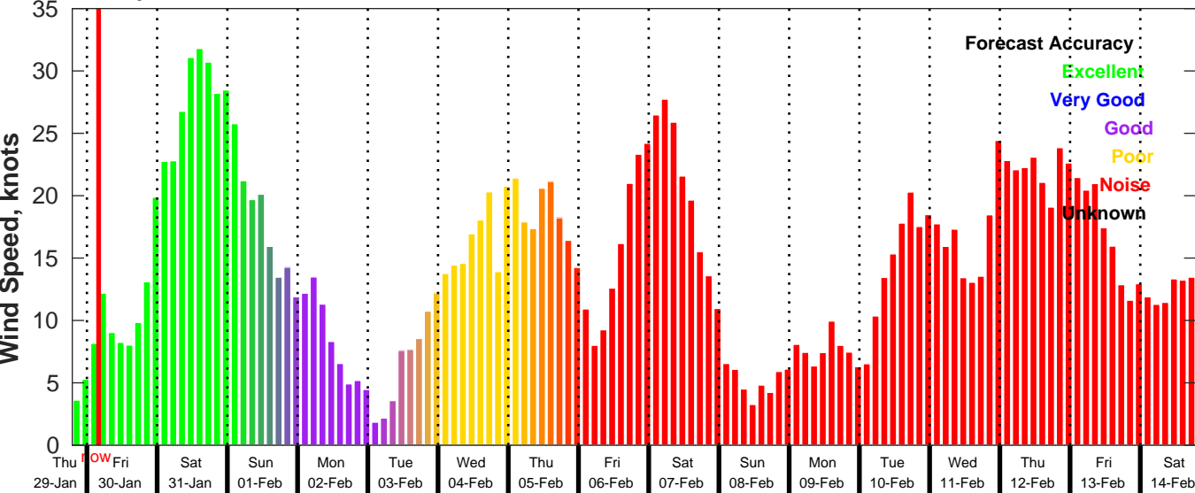
GFS Wind Speed Forecast for NDBC 42040 from 29-Jan-2026 19:00:00 to 14-Feb-2026 19:00:00
