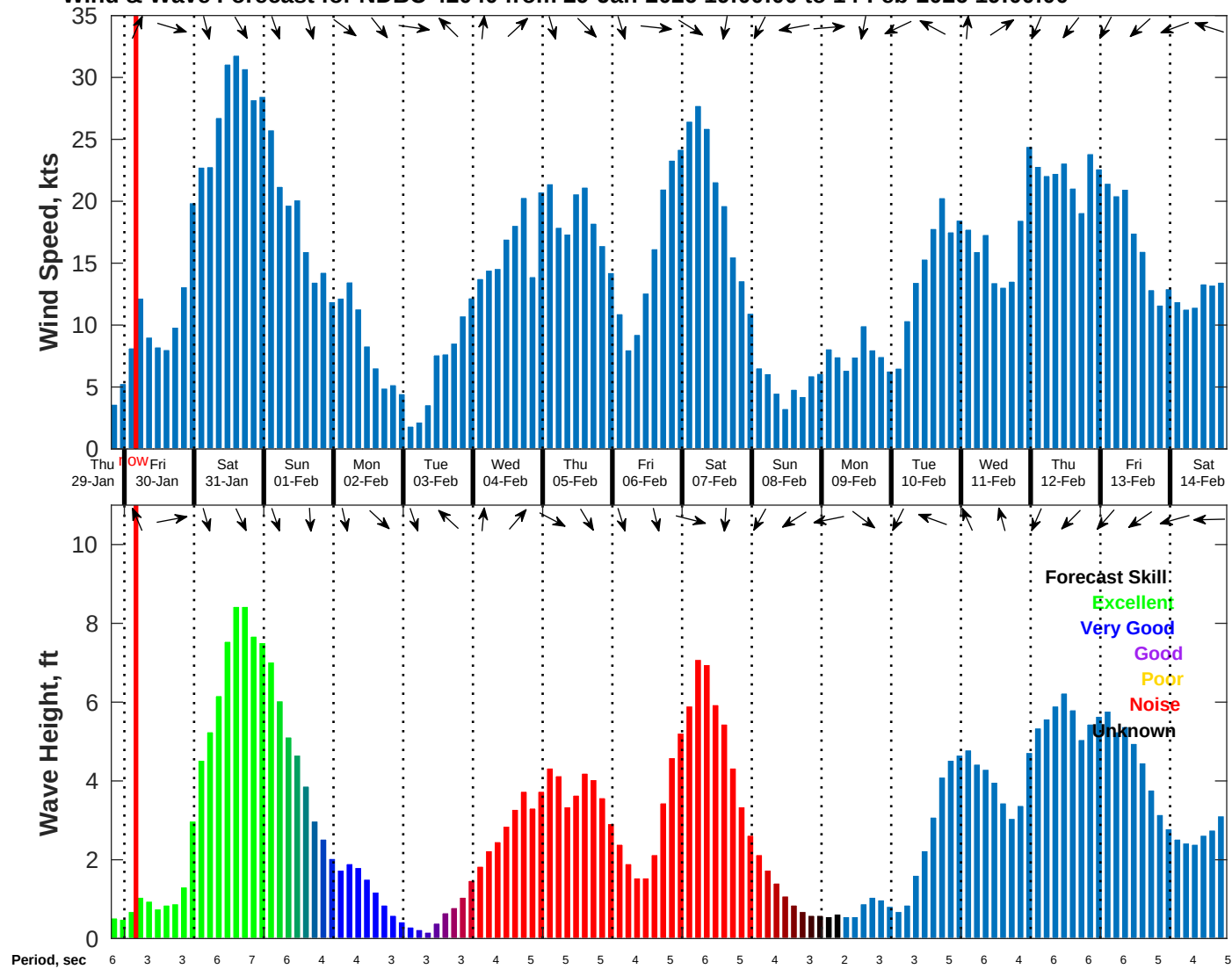
Wind & Wave Forecast for NDBC 42040 from 29-Jan-2026 19:00:00 to 14-Feb-2026 19:00:00
