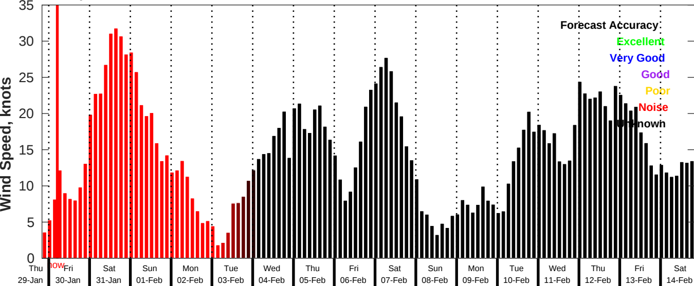
GFS Wind Speed Forecast for NDBC 42058 from 29-Jan-2026 20:00:00 to 14-Feb-2026 20:00:00
