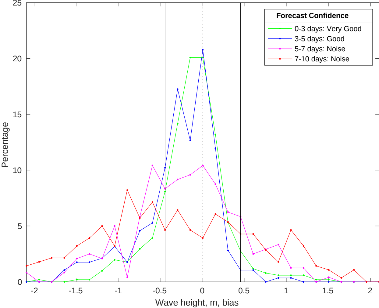
NDBC 44008 vs CMEMS Waves Bias Histogram: 30-Jan-2026
