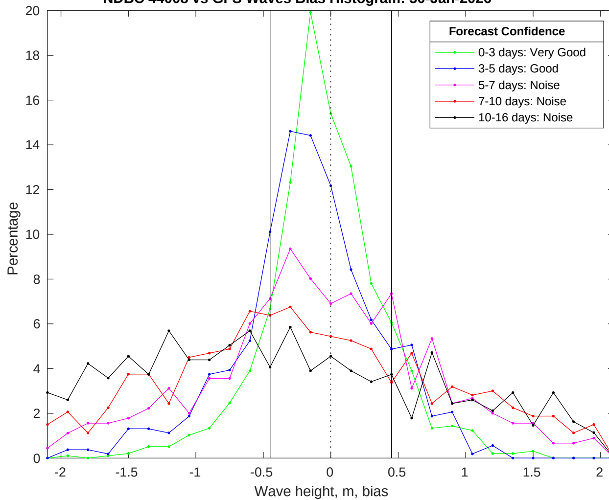
NDBC 44008 vs GFS Waves Bias Histogram: 30-Jan-2026
